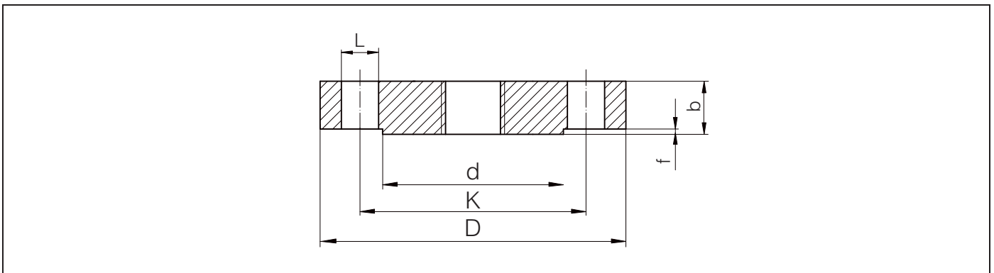
Fig. 14: Dimensions - ASME flange ANSI B 16.5 (seal ledge RF)
