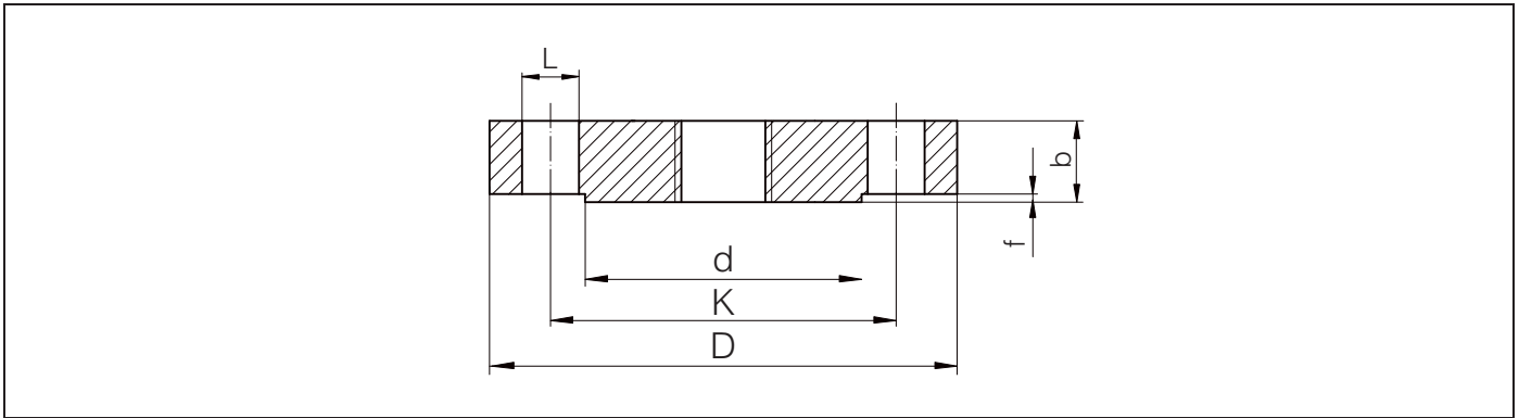
Fig. 21: Dimensions - JIS flange (Regular Flange)
